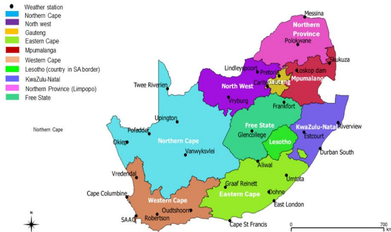
Figure 1.1 Geographical location of the 29 weather stations used in this study in all provinces of South Africa.
